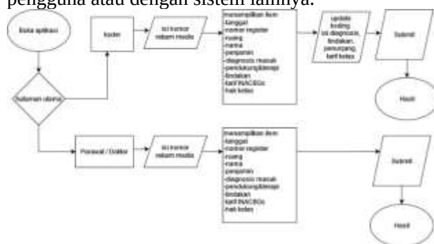
Gambar 2. Activity diagram
